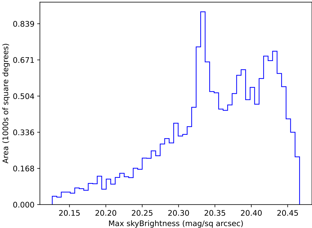
ddf_loaded_half_fl15_v3.4_10yrs WFD i band: Max skyBrightness
