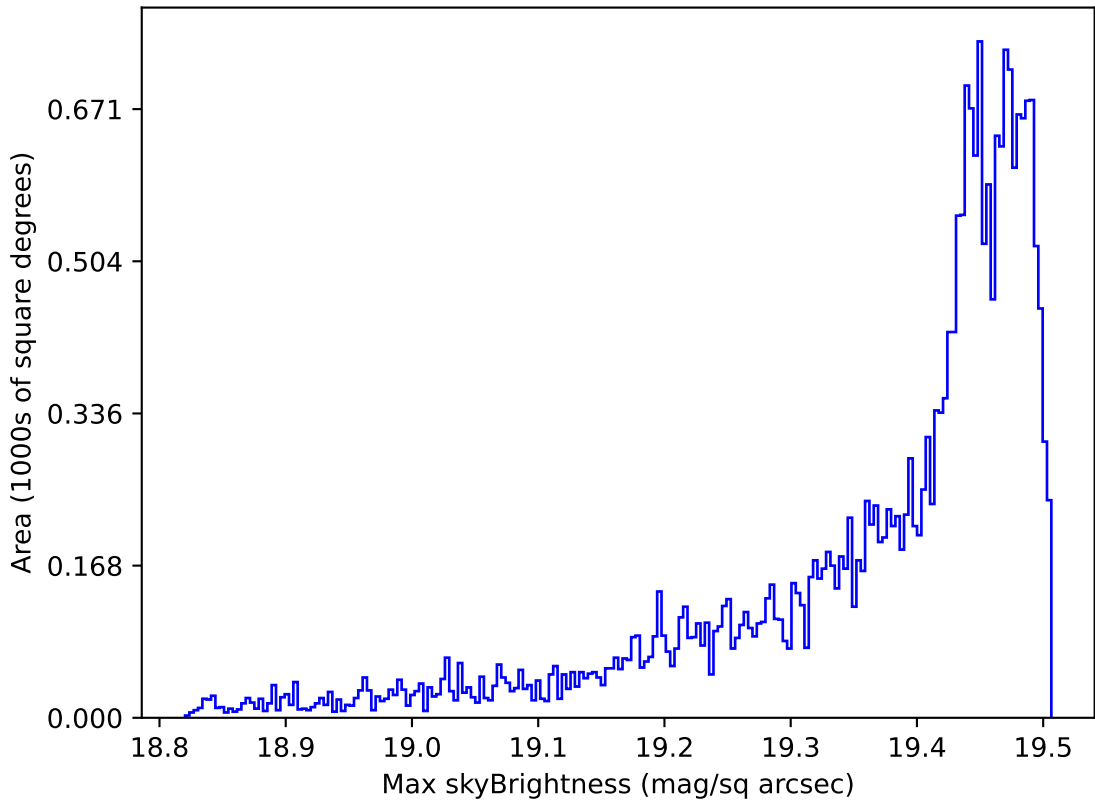
ddf_loaded_half_fl15_v3.4_10yrs All sky z band: Max skyBrightness
