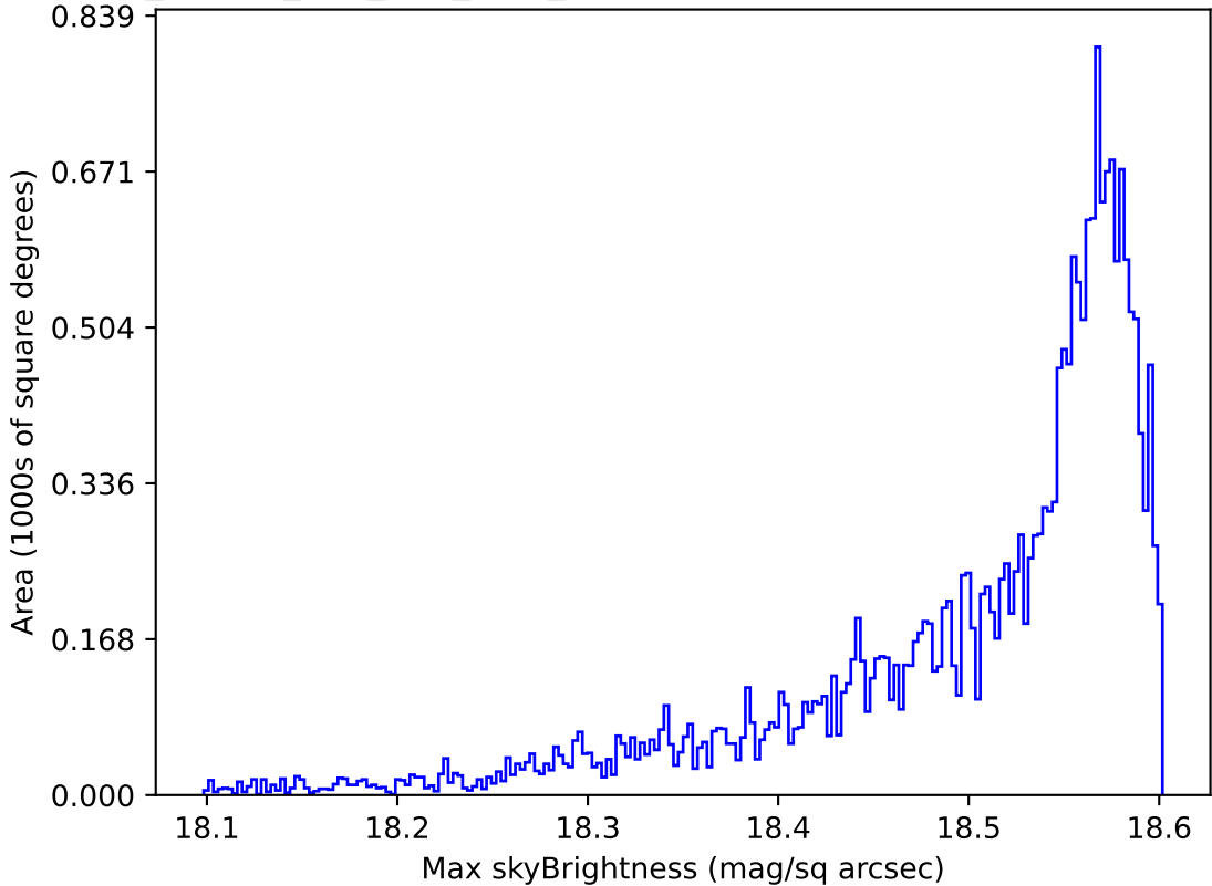
ddf_loaded_half_fl15_v3.4_10yrs All sky y band: Max skyBrightness
