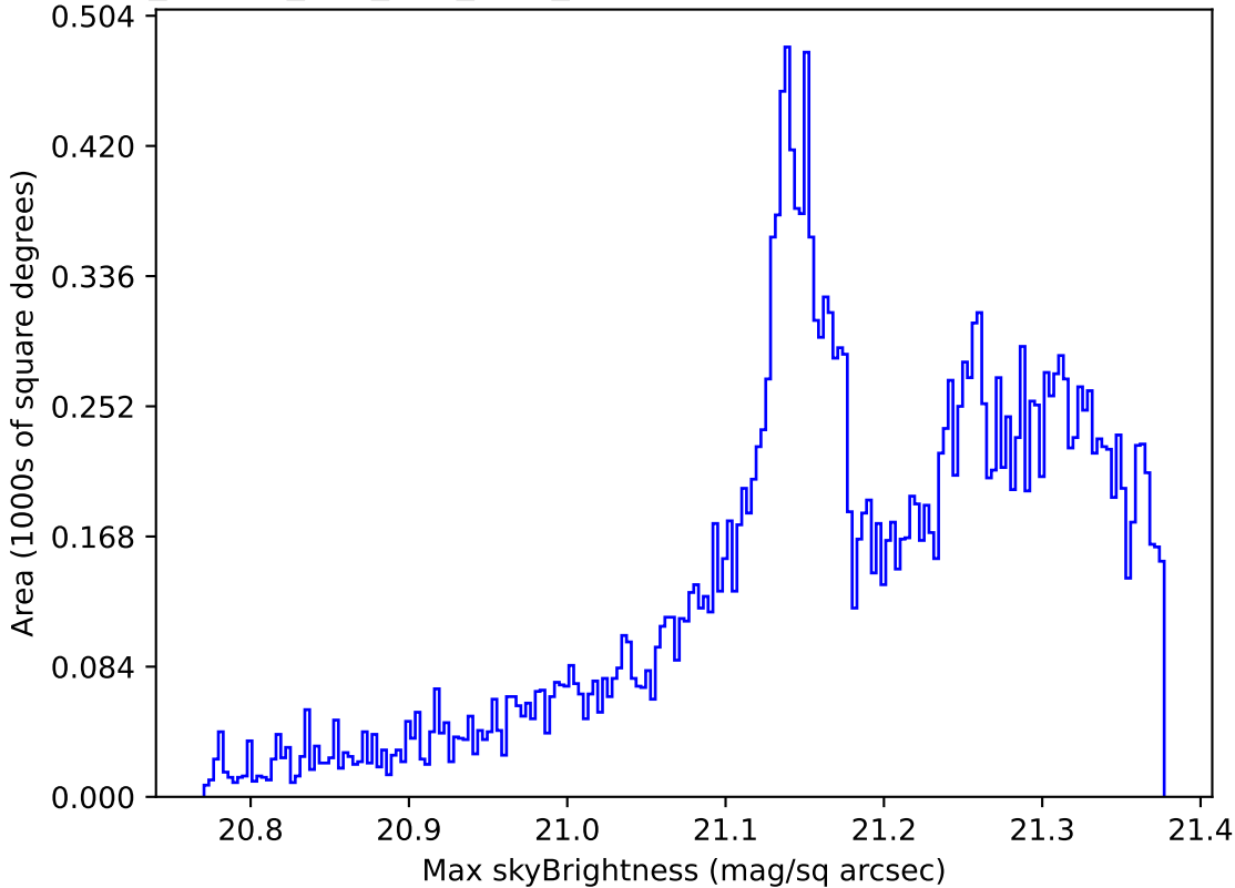
ddf_loaded_half_fl15_v3.4_10yrs All sky r band: Max skyBrightness
