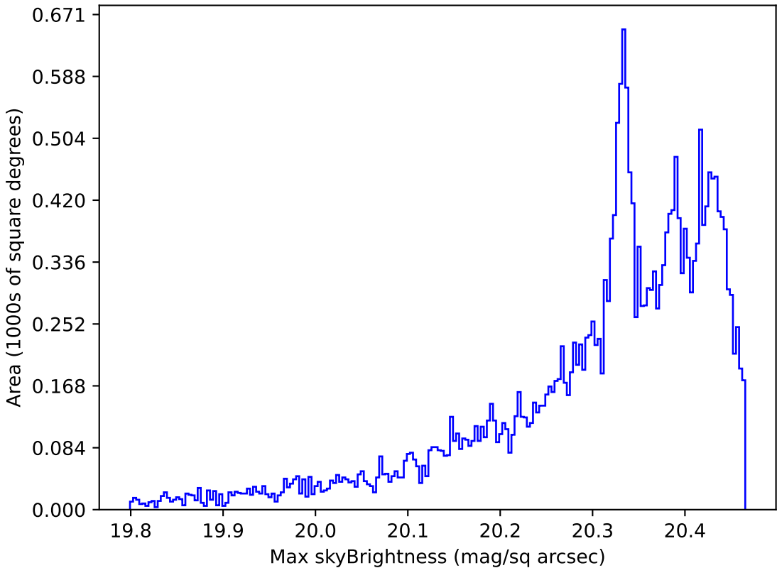
ddf_loaded_half_f15_v3.4_10yrs All sky i band: Max skyBrightness
