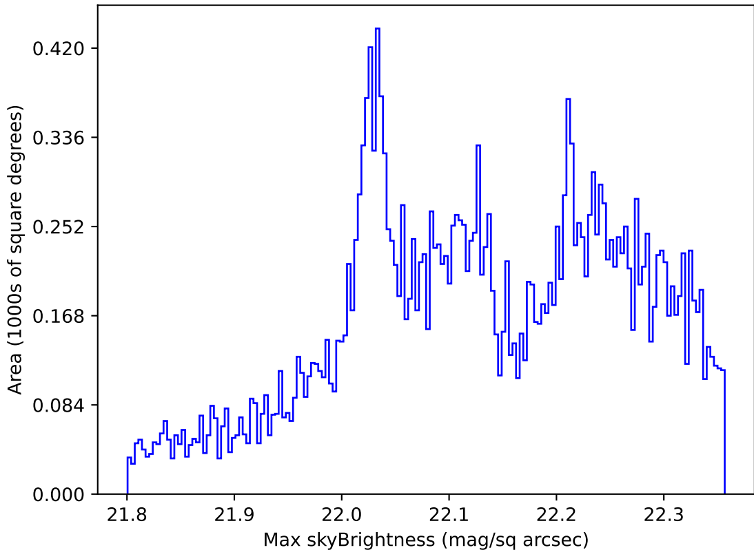
ddf_loaded_half_fl15_v3.4_10yrs All sky g band: Max skyBrightness
