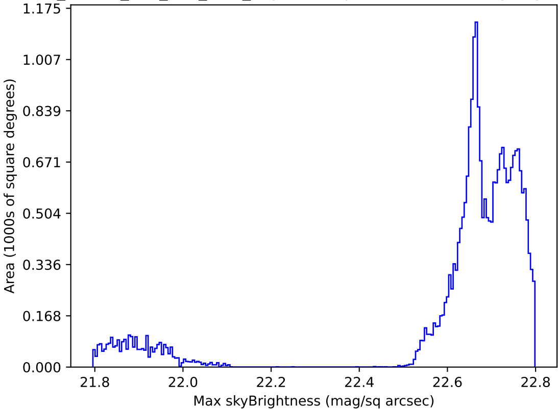
ddf_loaded_half_fl15_v3.4_10yrs All sky all bands: Max skyBrightness
