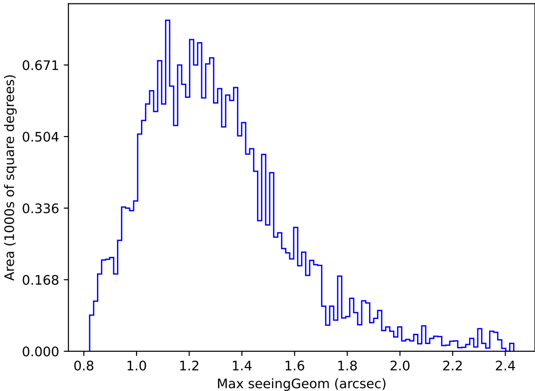
ddf_loaded_half_fl15_v3.4_10yrs Yr 1 z band: Max seeingGeom
