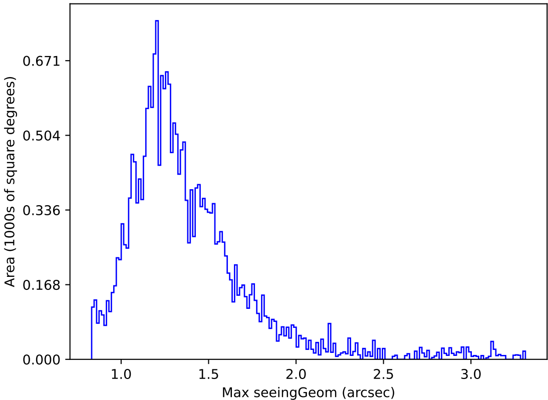
ddf_loaded_half_fl15_v3.4_10yrs Yr 1 u band: Max seeingGeom
