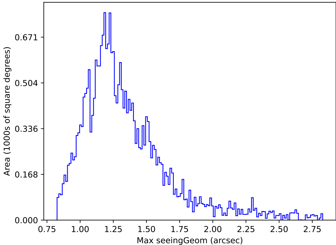
ddf_loaded_half_fl15_v3.4_10yrs Yr 1 i band: Max seeingGeom
