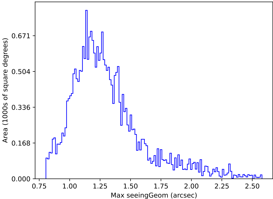
ddf_loaded_half_fl15_v3.4_10yrs Yr 1 g band: Max seeingGeom
