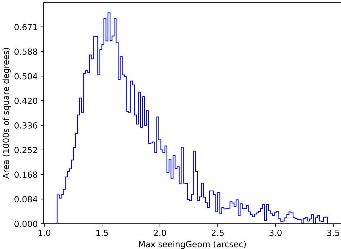
ddf_loaded_half_fl15_v3.4_10yrs Yr 1 all bands: Max seeingGeom
