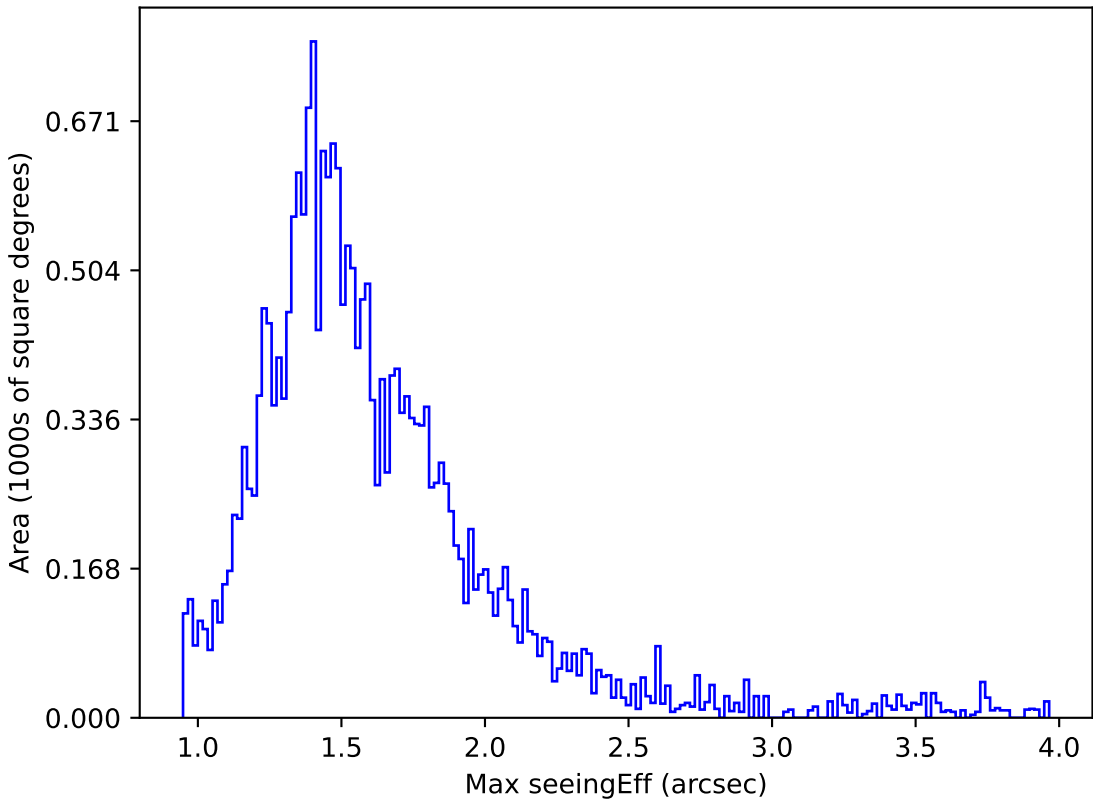
ddf_loaded_half_fl15_v3.4_10yrs Yr 1 u band: Max seeingEff
