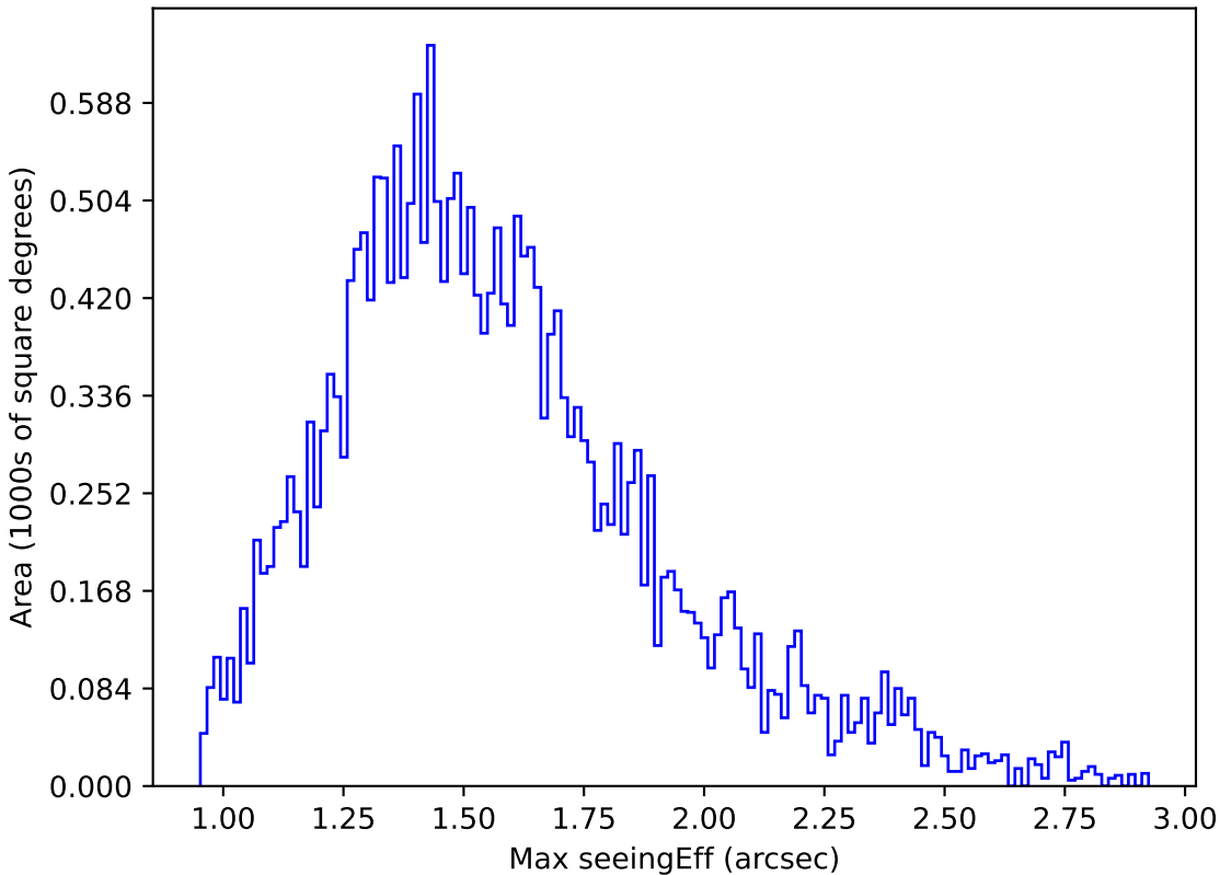
ddf_loaded_half_fl15_v3.4_10yrs Yr 1 r band: Max seeingEff
