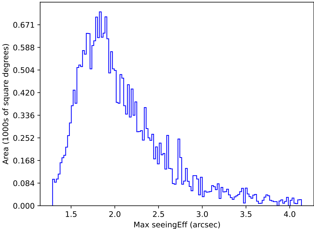
ddf_loaded_half_fl15_v3.4_10yrs Yr 1 all bands: Max seeingEff
