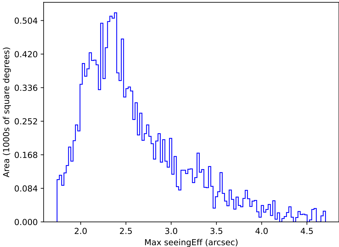
ddf_loaded_half_fl15_v3.4_10yrs WFD u band: Max seeingEff
