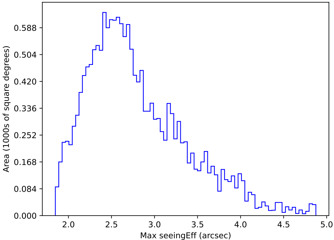
ddf_loaded_half_fl15_v3.4_10yrs WFD r band: Max seeingEff
