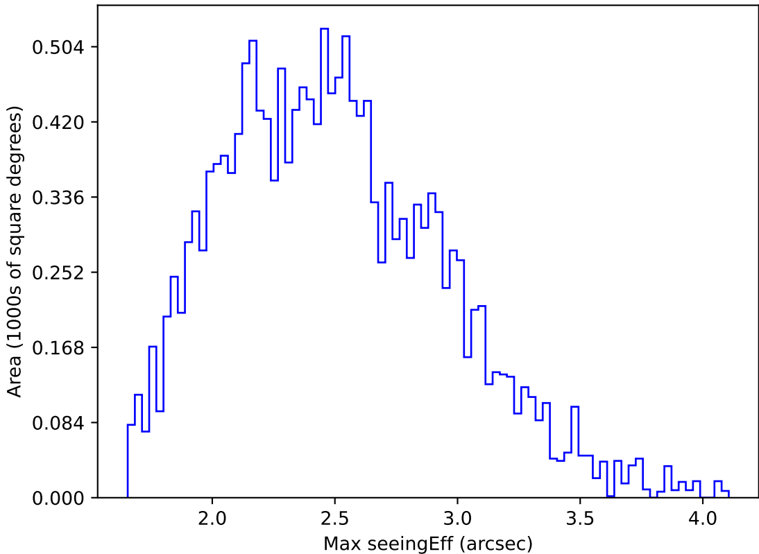
ddf_loaded_half_fl15_v3.4_10yrs WFD g band: Max seeingEff
