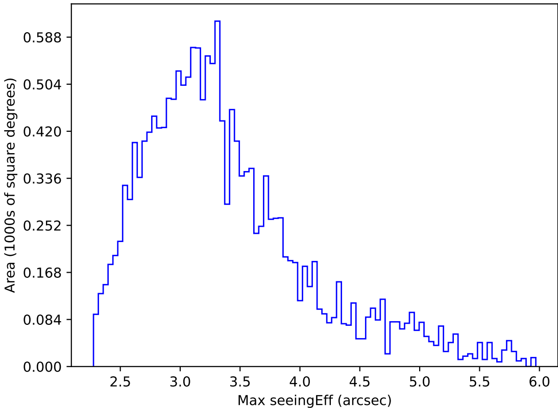
ddf_loaded_half_fl15_v3.4_10yrs WFD all bands: Max seeingEff
