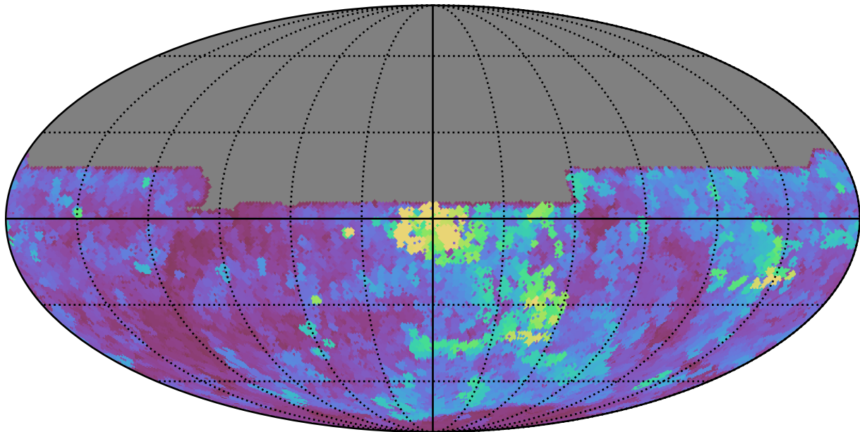
ddf_loaded_half_fl15_v3.4_10yrs All sky y band: Max seeingEff
