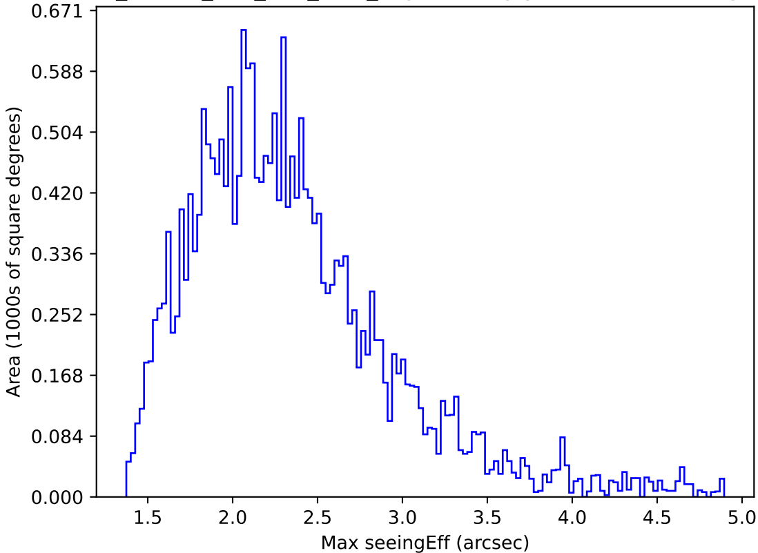
ddf_loaded_half_fl15_v3.4_10yrs All sky y band: Max seeingEff
