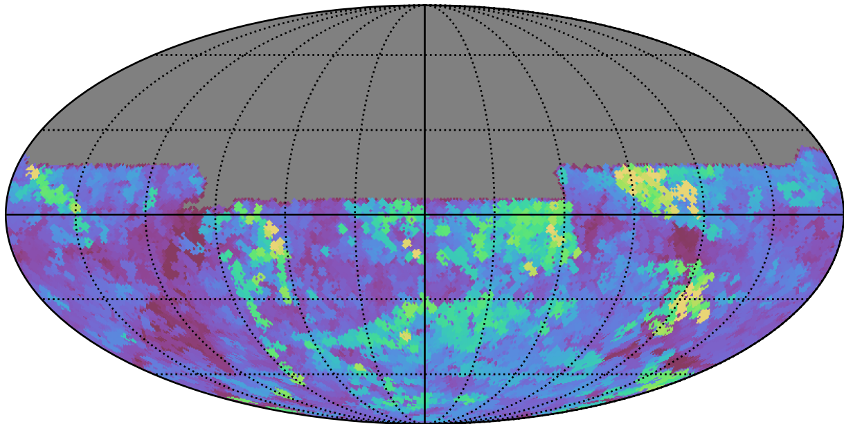
ddf_loaded_half_fl15_v3.4_10yrs All sky u band: Max seeingEff
