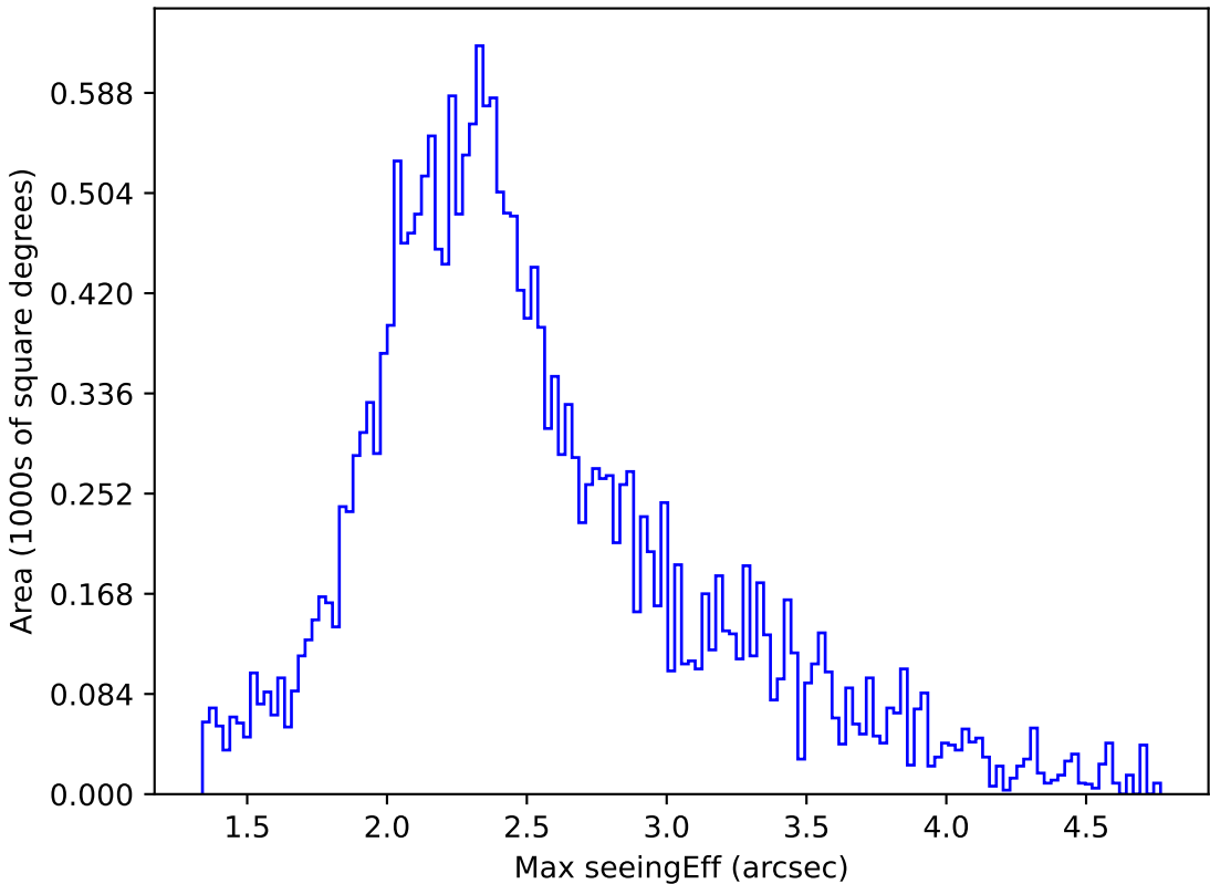
ddf_loaded_half_fl15_v3.4_10yrs All sky u band: Max seeingEff
