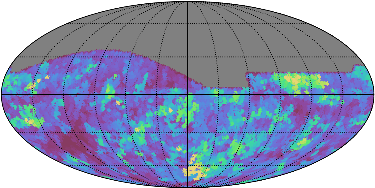
ddf_loaded_half_fl15_v3.4_10yrs All sky r band: Max seeingEff
