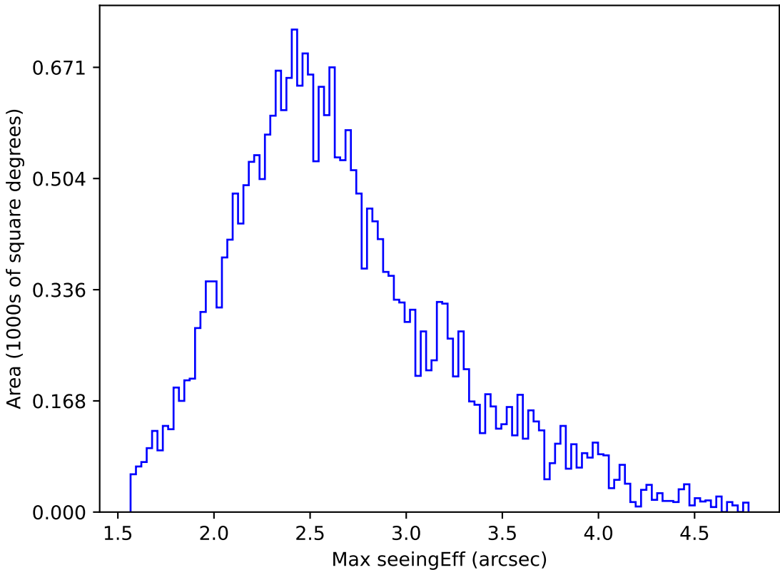
ddf_loaded_half_fl15_v3.4_10yrs All sky r band: Max seeingEff
