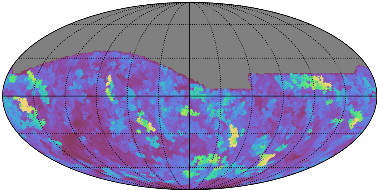
ddf_loaded_half_fl15_v3.4_10yrs All sky i band: Max seeingEff
