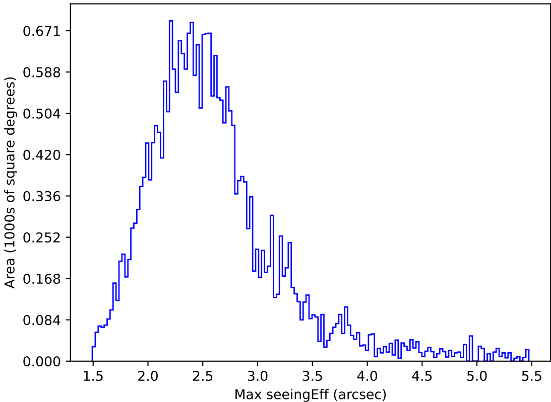
ddf_loaded_half_fl15_v3.4_10yrs All sky i band: Max seeingEff
