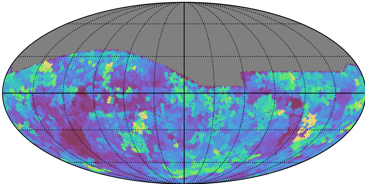
ddf_loaded_half_fl15_v3.4_10yrs All sky g band: Max seeingEff
