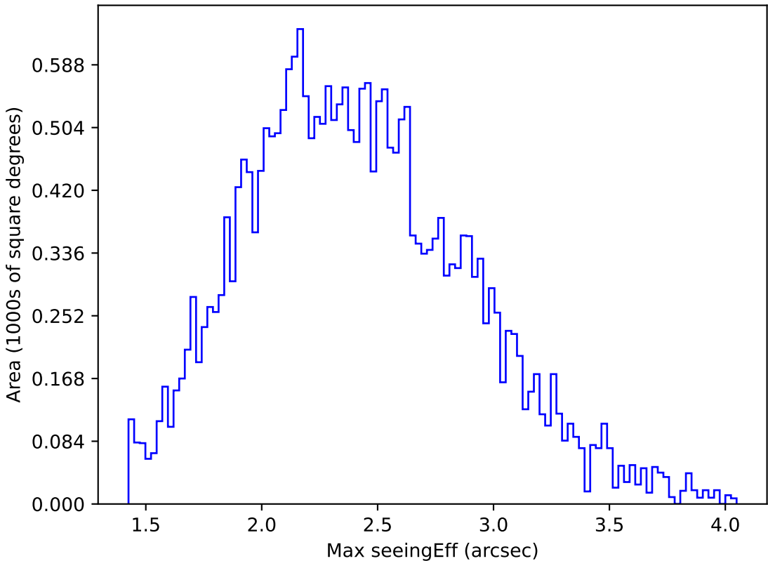
ddf_loaded_half_fl15_v3.4_10yrs All sky g band: Max seeingEff
