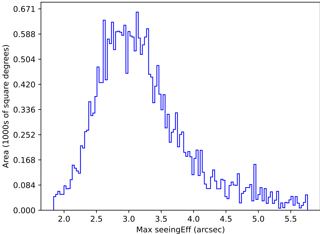
ddf_loaded_half_fl15_v3.4_10yrs All sky all bands: Max seeingEff
