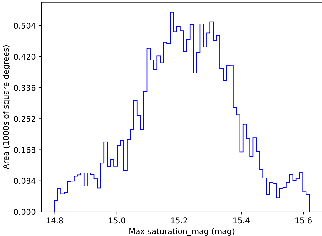
ddf_loaded_half_fl15_v3.4_10yrs WFD z band: Max saturation_mag
