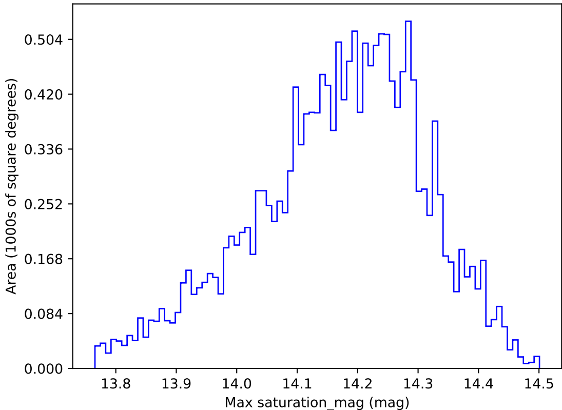
ddf_loaded_half_fl15_v3.4_10yrs WFD y band: Max saturation_mag
