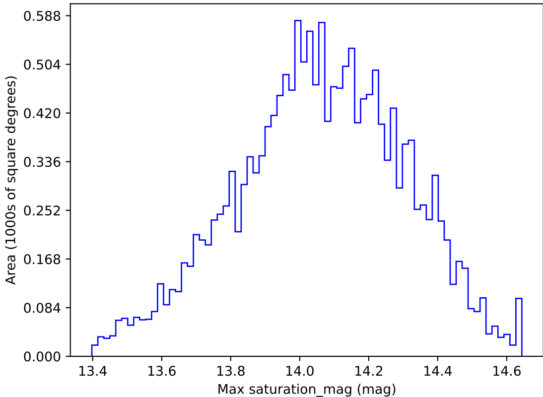
ddf_loaded_half_fl15_v3.4_10yrs WFD u band: Max saturation_mag
