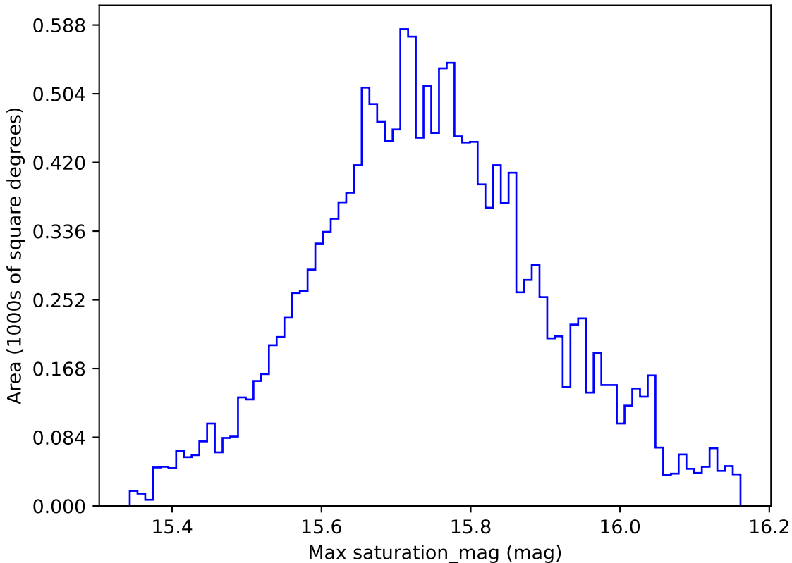
ddf_loaded_half_fl15_v3.4_10yrs WFD r band: Max saturation_mag
