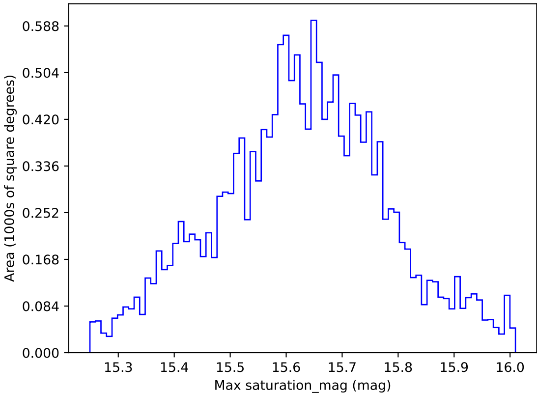
ddf_loaded_half_fl15_v3.4_10yrs WFD i band: Max saturation_mag
