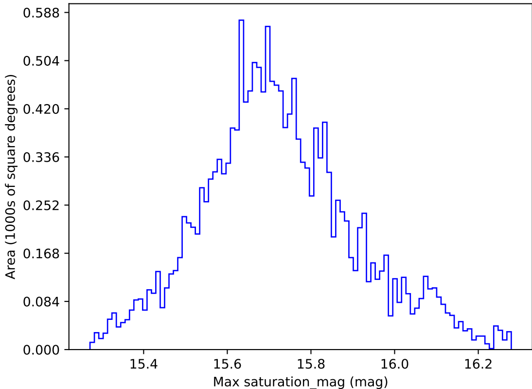
ddf_loaded_half_fl15_v3.4_10yrs WFD g band: Max saturation_mag
