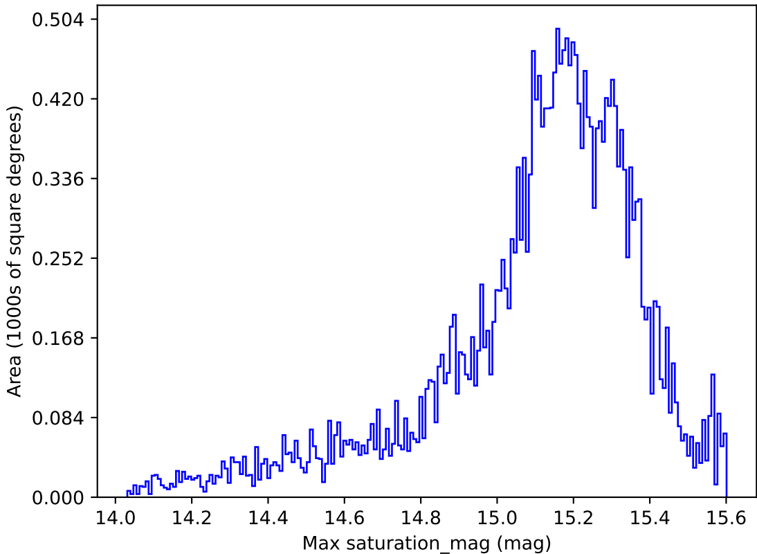
ddf_loaded_half_fl15_v3.4_10yrs All sky z band: Max saturation_mag
