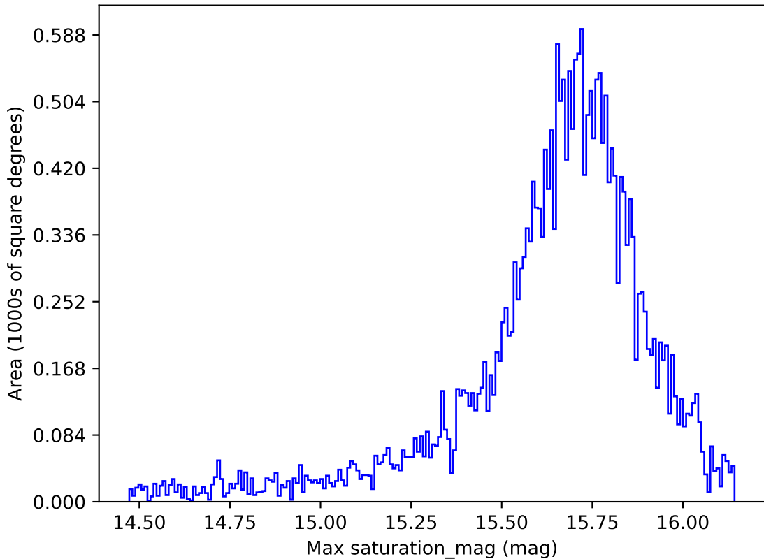
ddf_loaded_half_fl15_v3.4_10yrs All sky r band: Max saturation_mag
