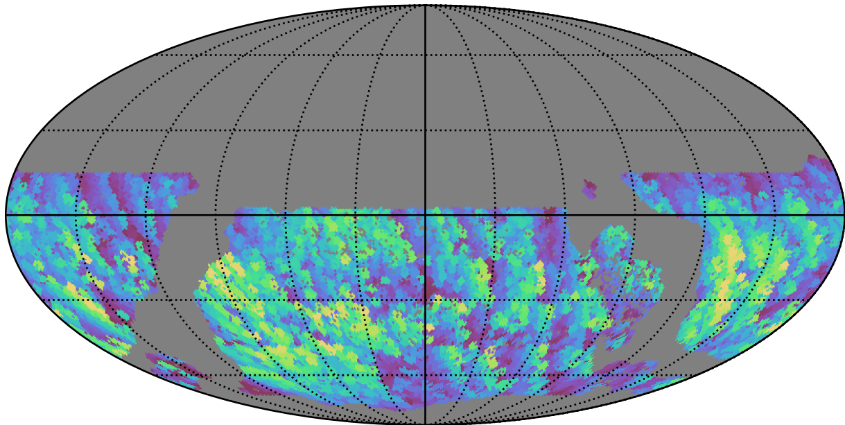
ddf_loaded_half_fl15_v3.4_10yrs WFD y band: Max normairmass
