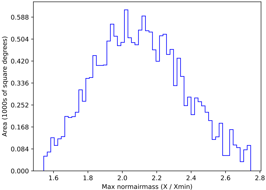
ddf_loaded_half_fl15_v3.4_10yrs WFD y band: Max normairmass
