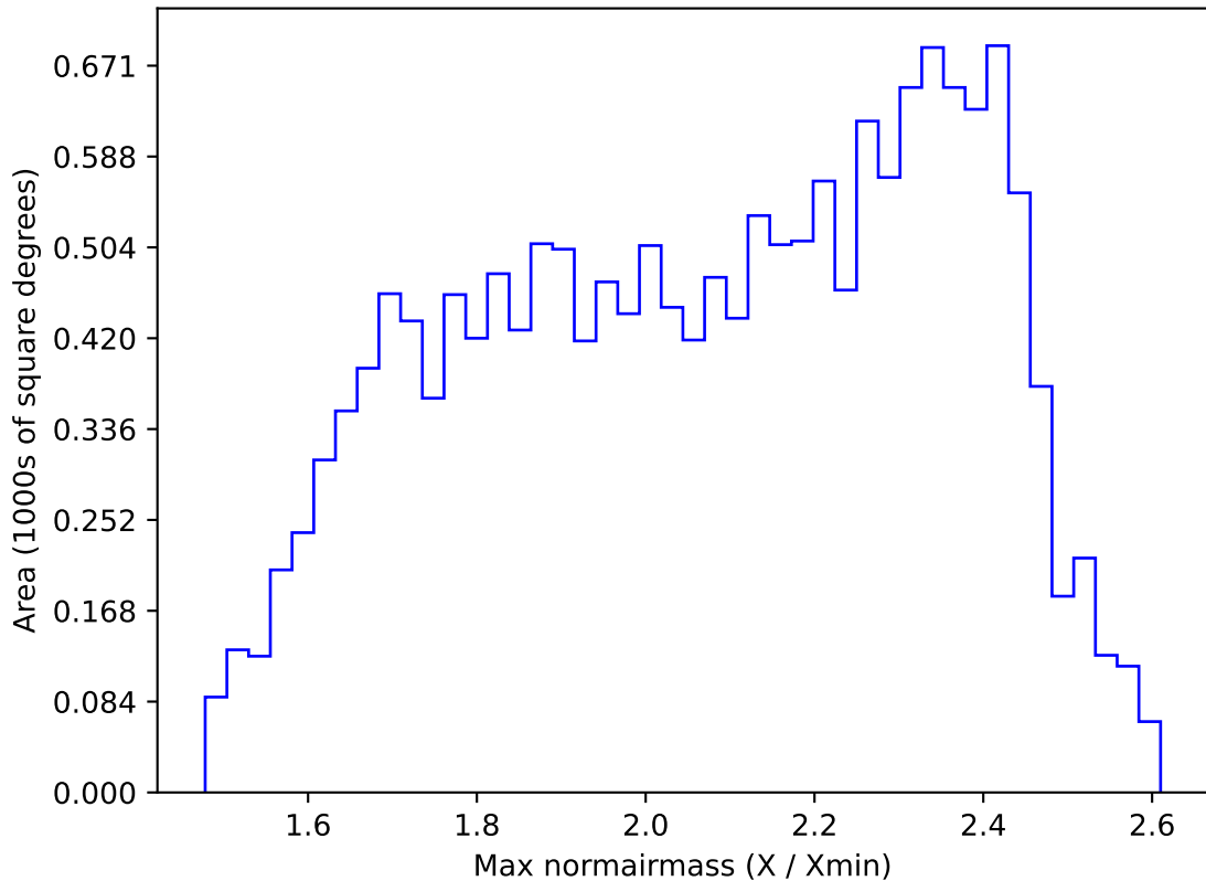
ddf_loaded_half_fl15_v3.4_10yrs WFD r band: Max normairmass
