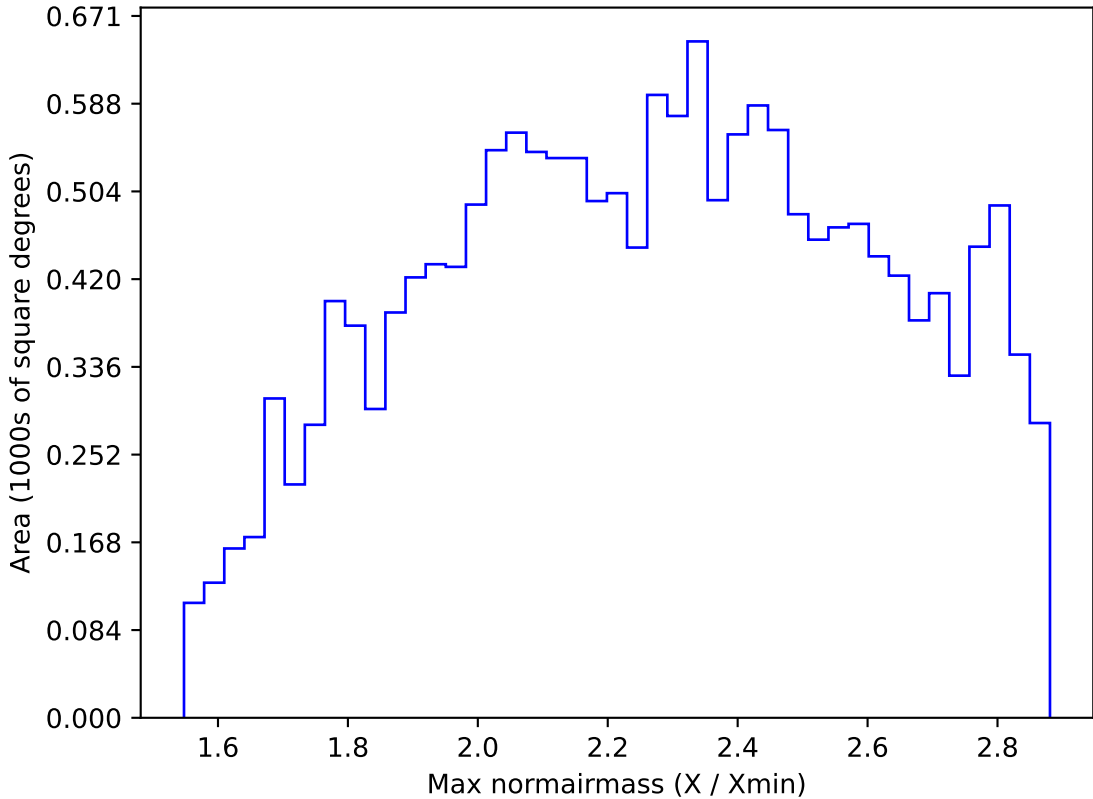
ddf_loaded_half_fl15_v3.4_10yrs WFD i band: Max normairmass
