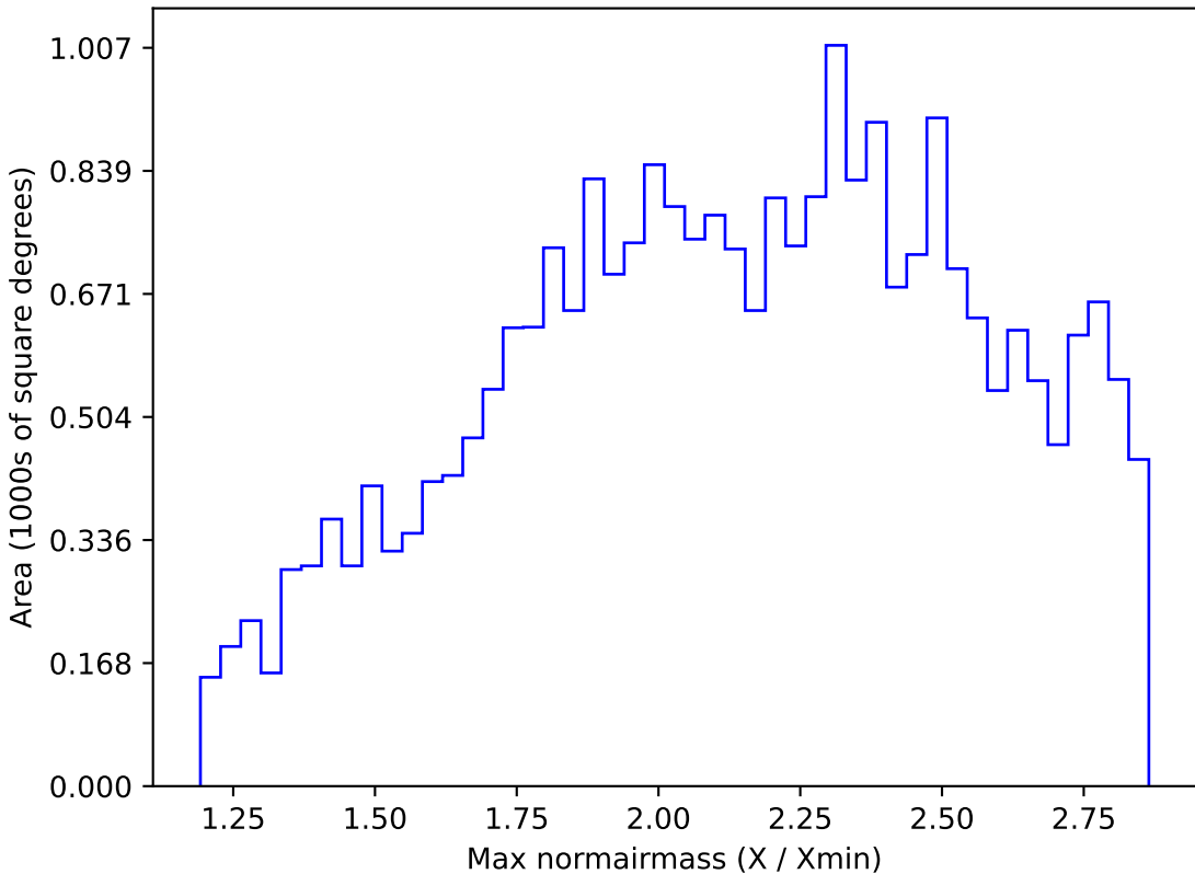
ddf_loaded_half_fl15_v3.4_10yrs All sky z band: Max normairmass
