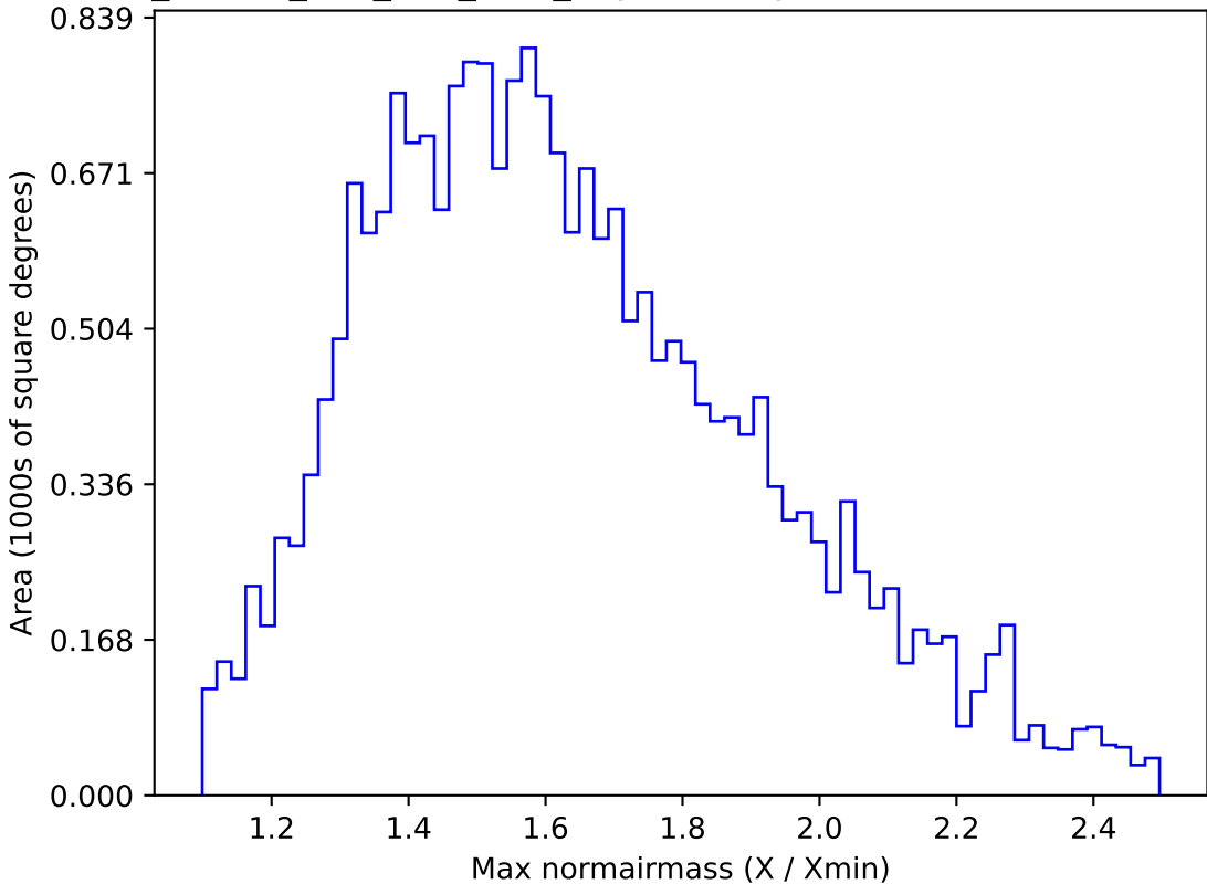
ddf_loaded_half_fl15_v3.4_10yrs All sky u band: Max normairmass
