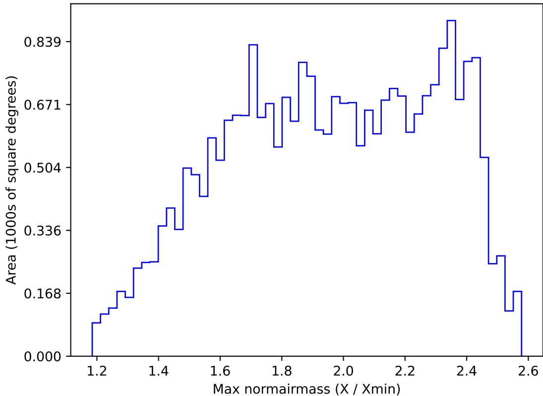
ddf_loaded_half_fl15_v3.4_10yrs All sky r band: Max normairmass
