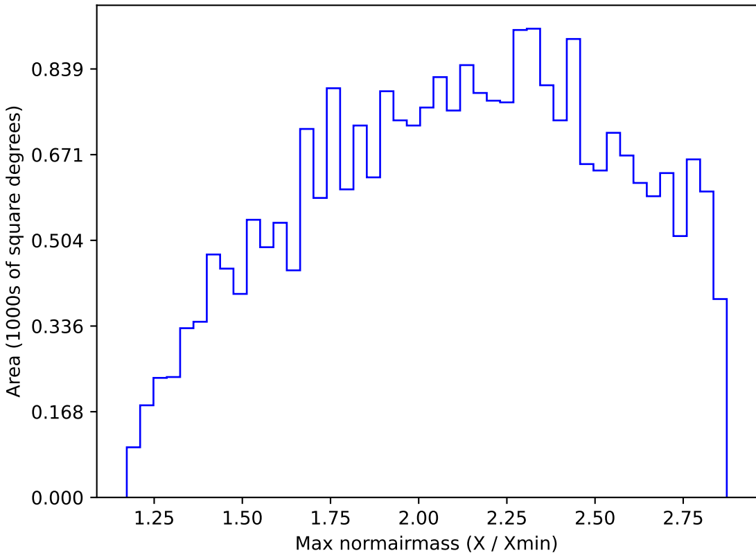
ddf_loaded_half_fl15_v3.4_10yrs All sky i band: Max normairmass
