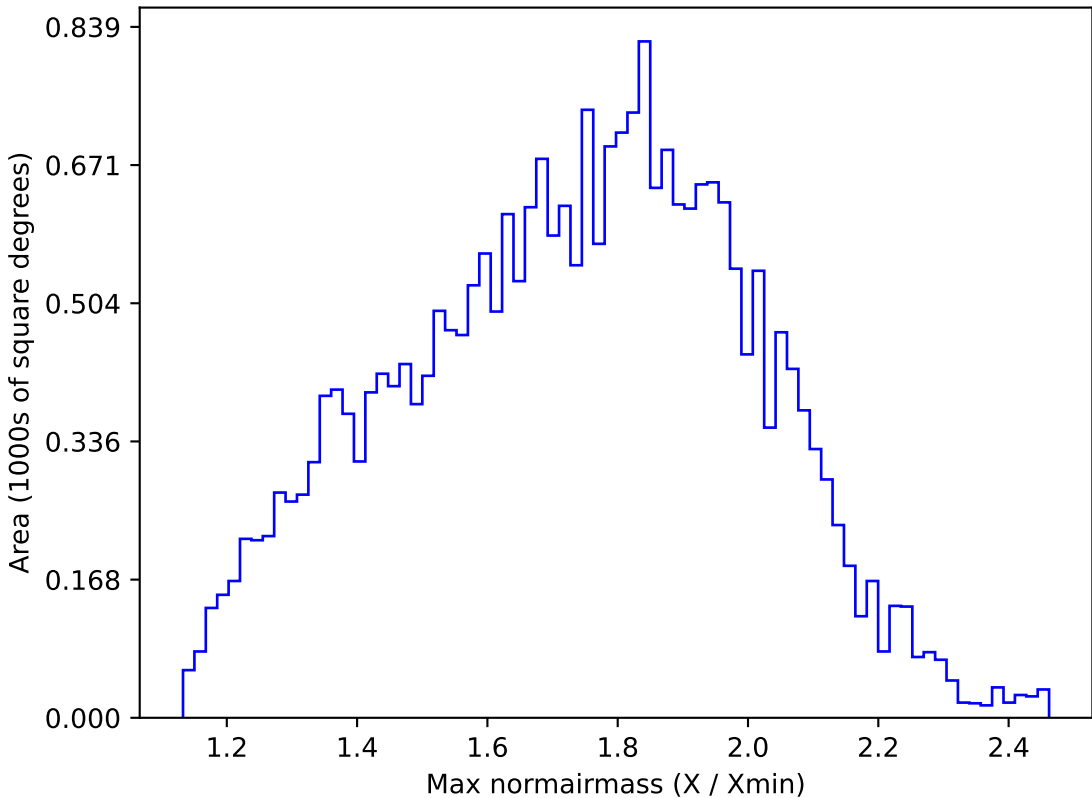
ddf_loaded_half_fl15_v3.4_10yrs All sky g band: Max normairmass
