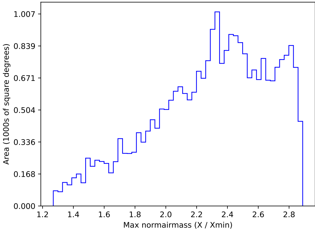
ddf_loaded_half_fl15_v3.4_10yrs All sky all bands: Max normairmass
