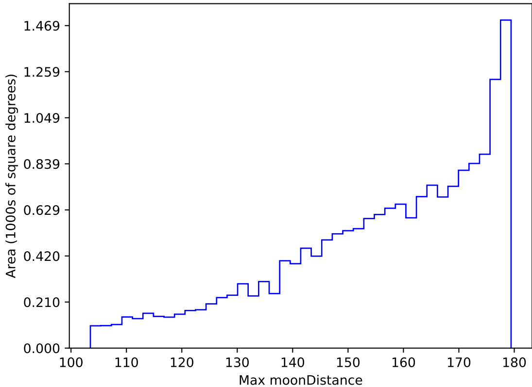
ddf_loaded_half_fl15_v3.4_10yrs WFD r band: Max moonDistance
