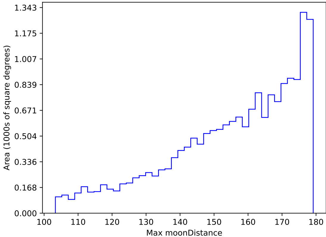
ddf_loaded_half_fl15_v3.4_10yrs WFD i band: Max moonDistance
